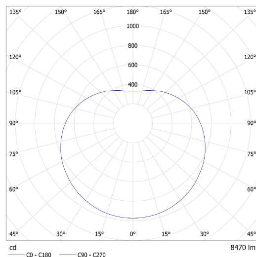
Lucis ZK.P4.600.X POLARIS ZK LED / LDC (Polar)
